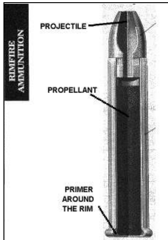
RIMFIRE CARTRIDGE
